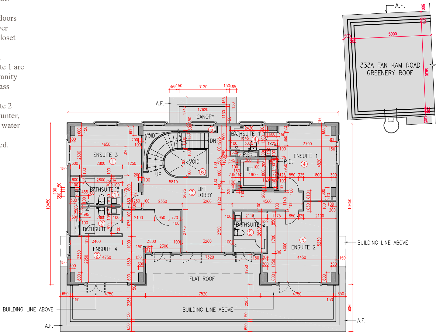
1/F AS IS FLOOR PLAN
