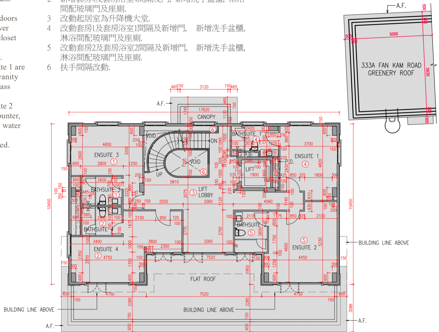
1/F AS IS FLOOR PLAN 1樓現狀平面圖
